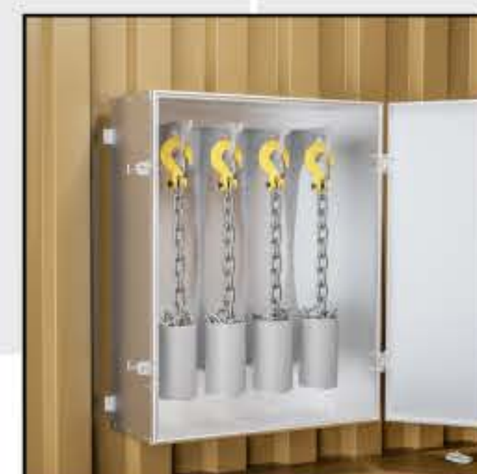
Storage for Lashing Equipment
